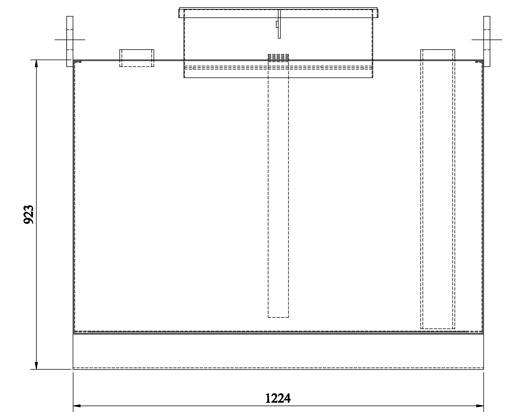
SIDE VIEW
